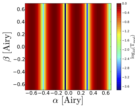
Figure 4.: theoretical normalized transfer function \bar{T}_{\text{theor}}^B(\alpha, \beta) , for \lambda = 2.45 \mu\text{m} .
