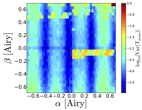
Figure 3.: variance of the measured normalized transfer function.
