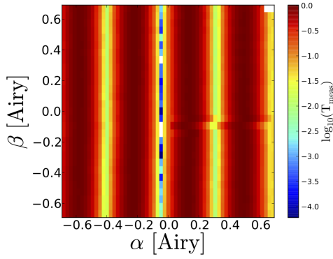
Figure 2.: measured normalized transfer function \bar{T}_{\text{meas}}^B(\alpha, \beta) for \lambda = 2.45 \mu\text{m} .
