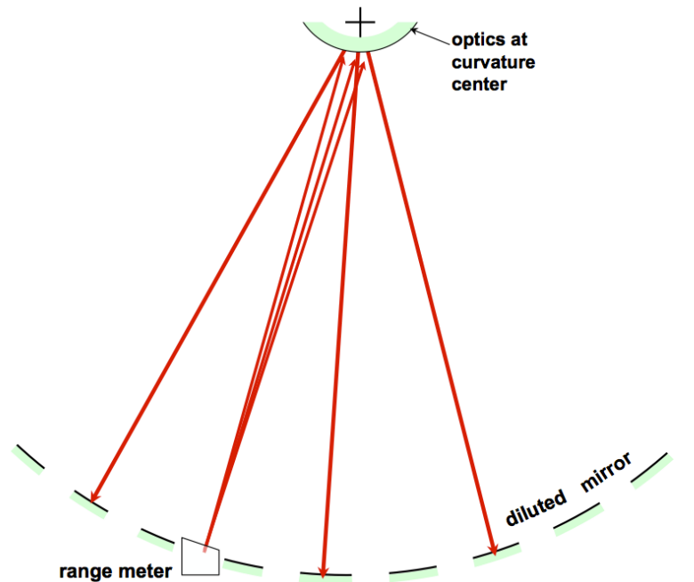
Figure 1.: Use of laser ranging for optical path equalization via the curvature center.
